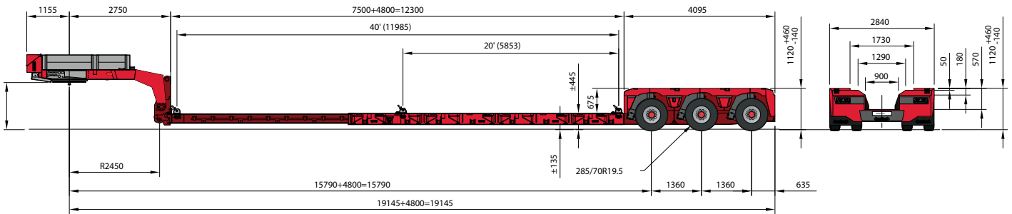
3-axle EURO-PX3: 285/70R19.5 tires
